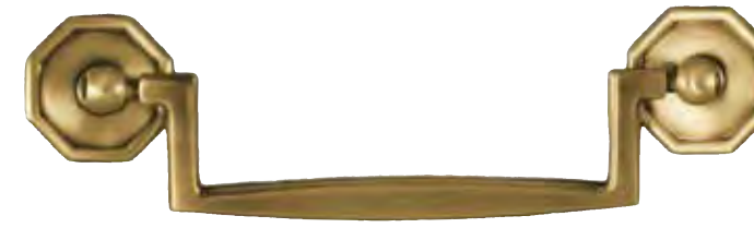
Bail Pull R1 W5¾ D¾ H2¼ (Boring 4½)
